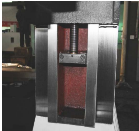
Z axes SWALLOW-TAIL shape hard guideway
