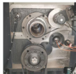
Hydraulic gear spindle
